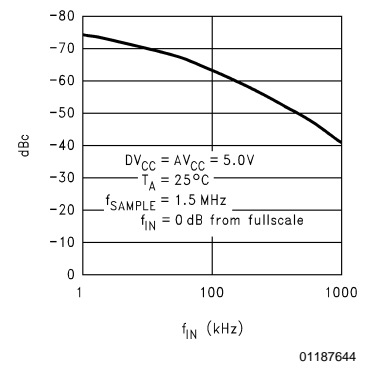
THD vs Input Frequency (Through Mux)
